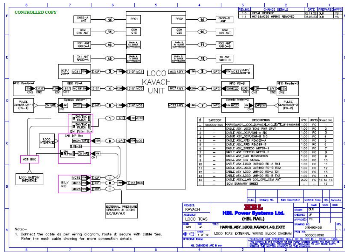
On Board Kavach block diagram
