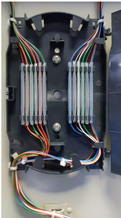
Station OFC Termination panel(Installation at site-In Inside)
