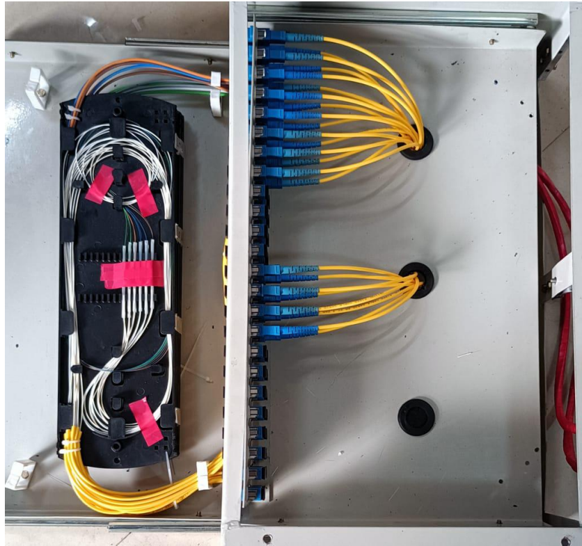
OFC Splicing in inside the OFC Termination unit(FDMS)
