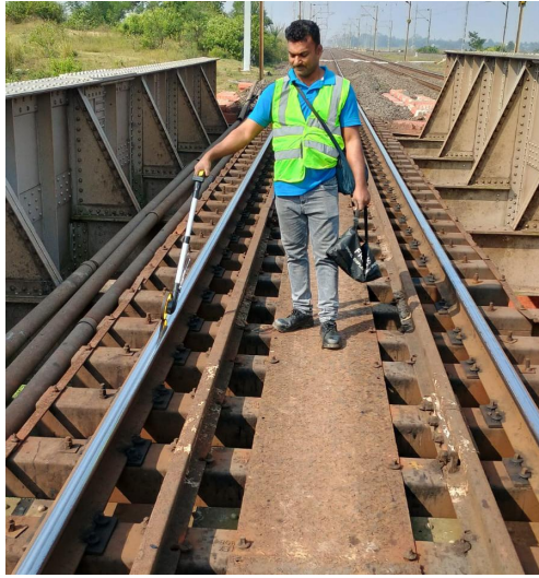
RFID TAG fixing as Layout plan at site
