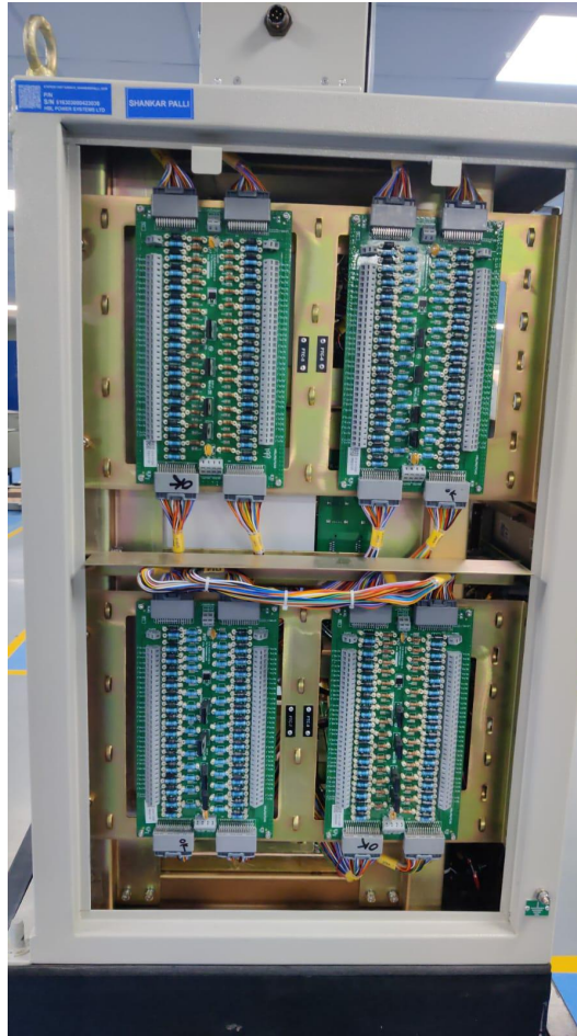
Field unit termination in Stationary kavach in Relay room
