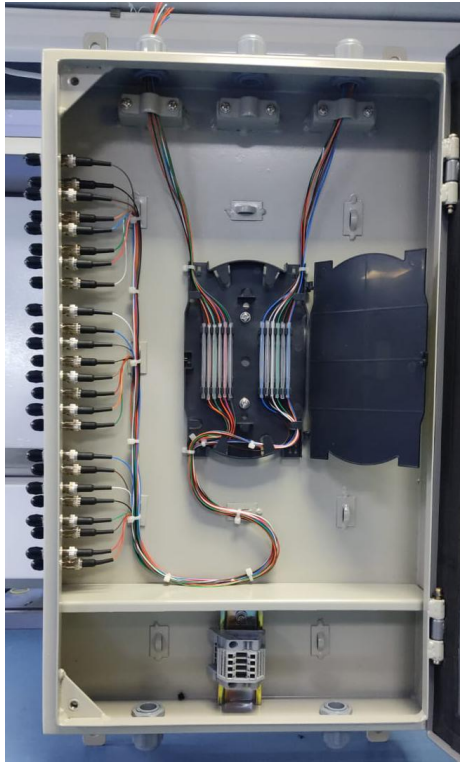
Station OFC Termination panel(Installation at site-In Inside)
