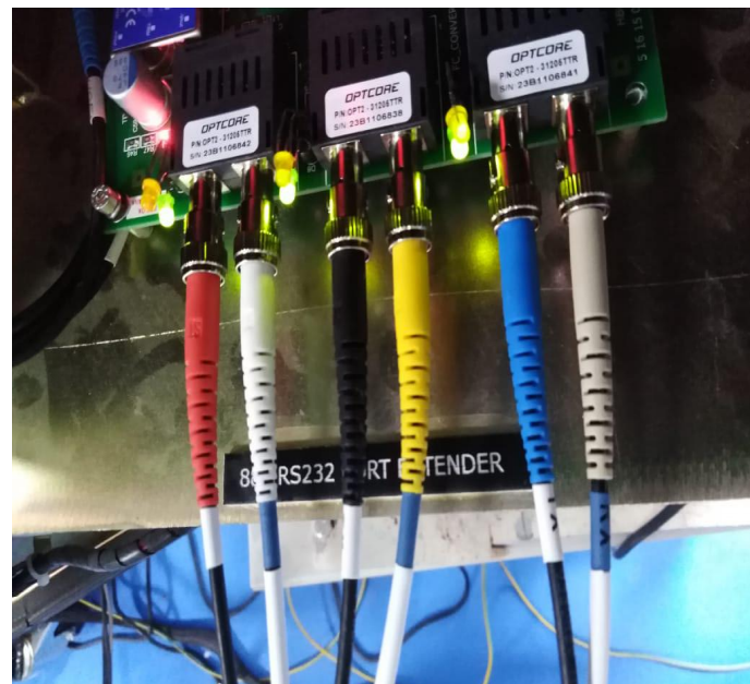
OFC Terminations in RTU Tower side in inside at RS232 -OFC Converter
