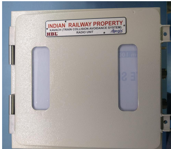
Radio unit(Front View)
