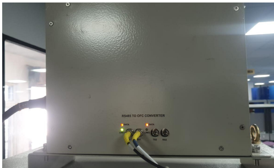
Station master operation and indication panel(Rear View)
